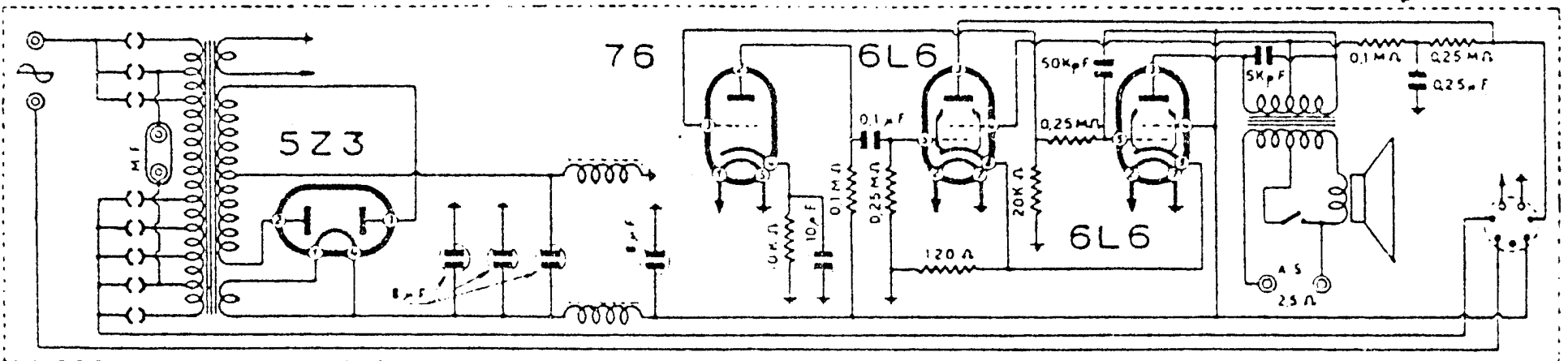
UNDO RADIO - MOD. « SUPER QUADRI UNDA 838 »
